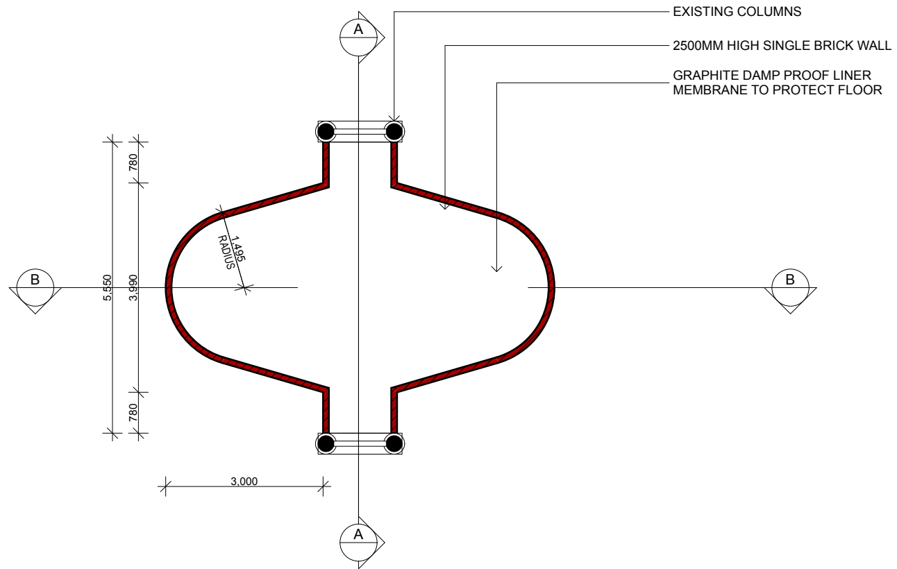
1 FLOOR PLAN 1:100
